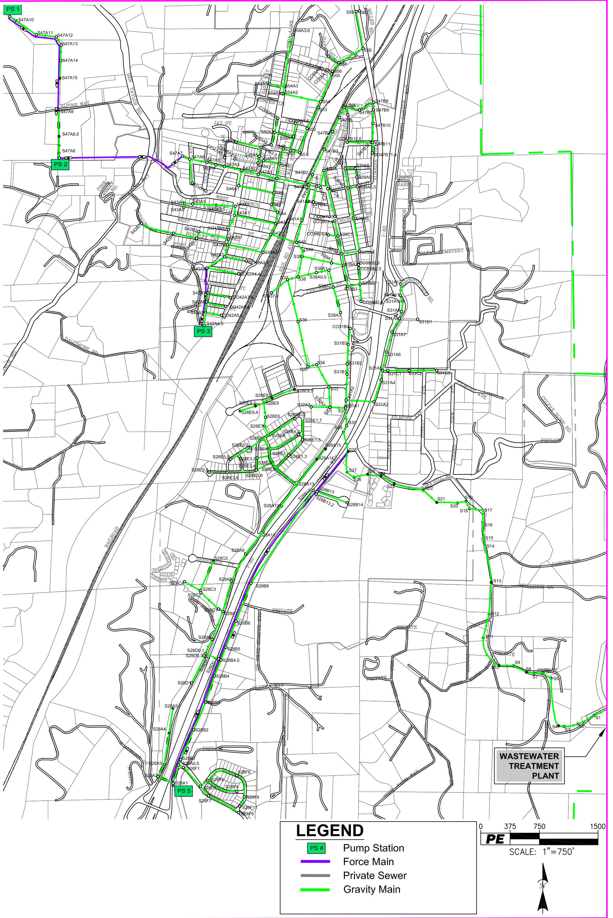
FIGURE 2: COLFAX SEWER COLLECTION SYSTEM MAP
